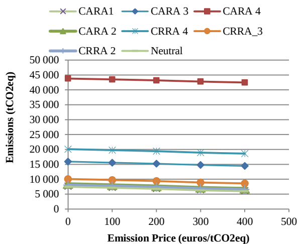
A. Evolution of emissions under different risk scenari
